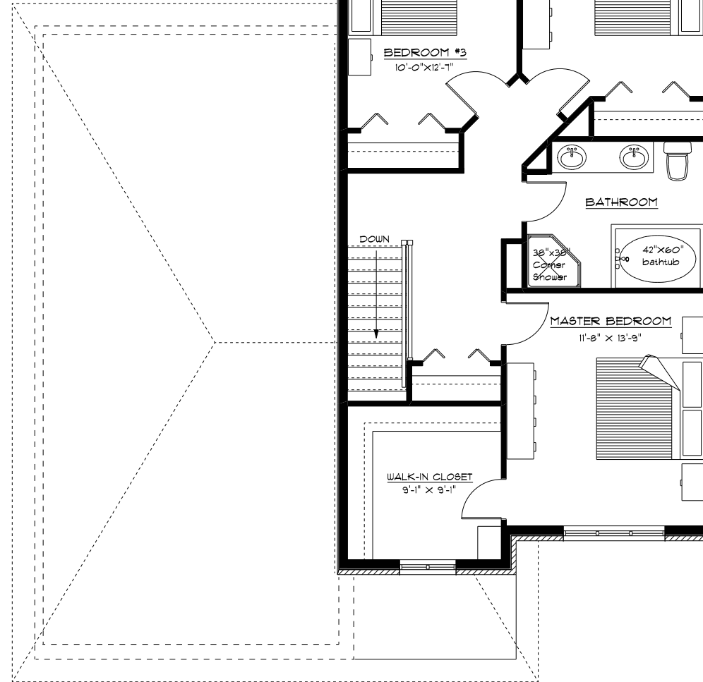
2ND FLOOR PLAN 834 sq.ft
