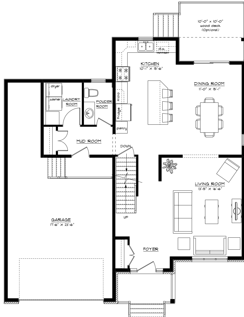
GROUND FLOOR PLAN 947 sq.ft
