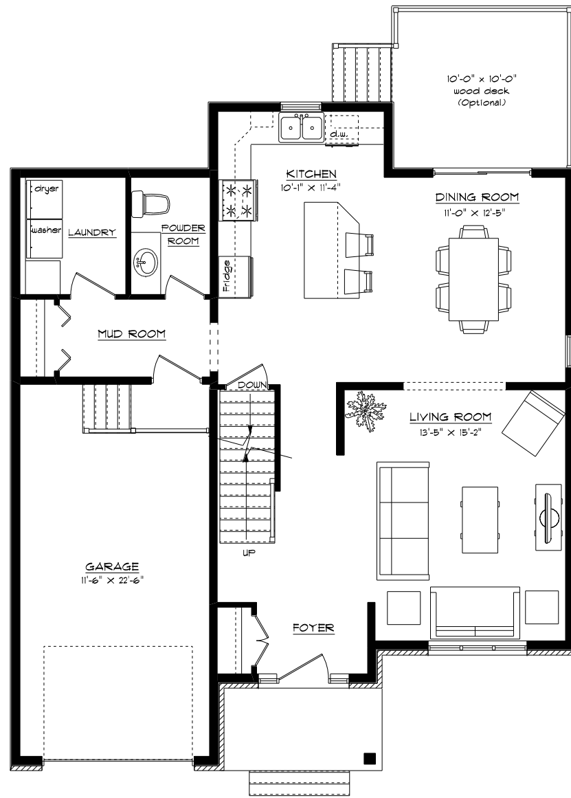
GROUND FLOOR PLAN 859 sq.ft
