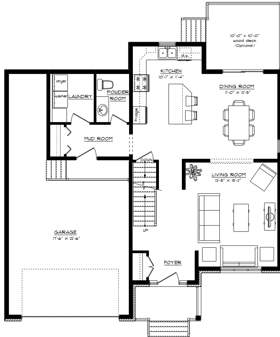
GROUND FLOOR PLAN 859 sq.ft.
