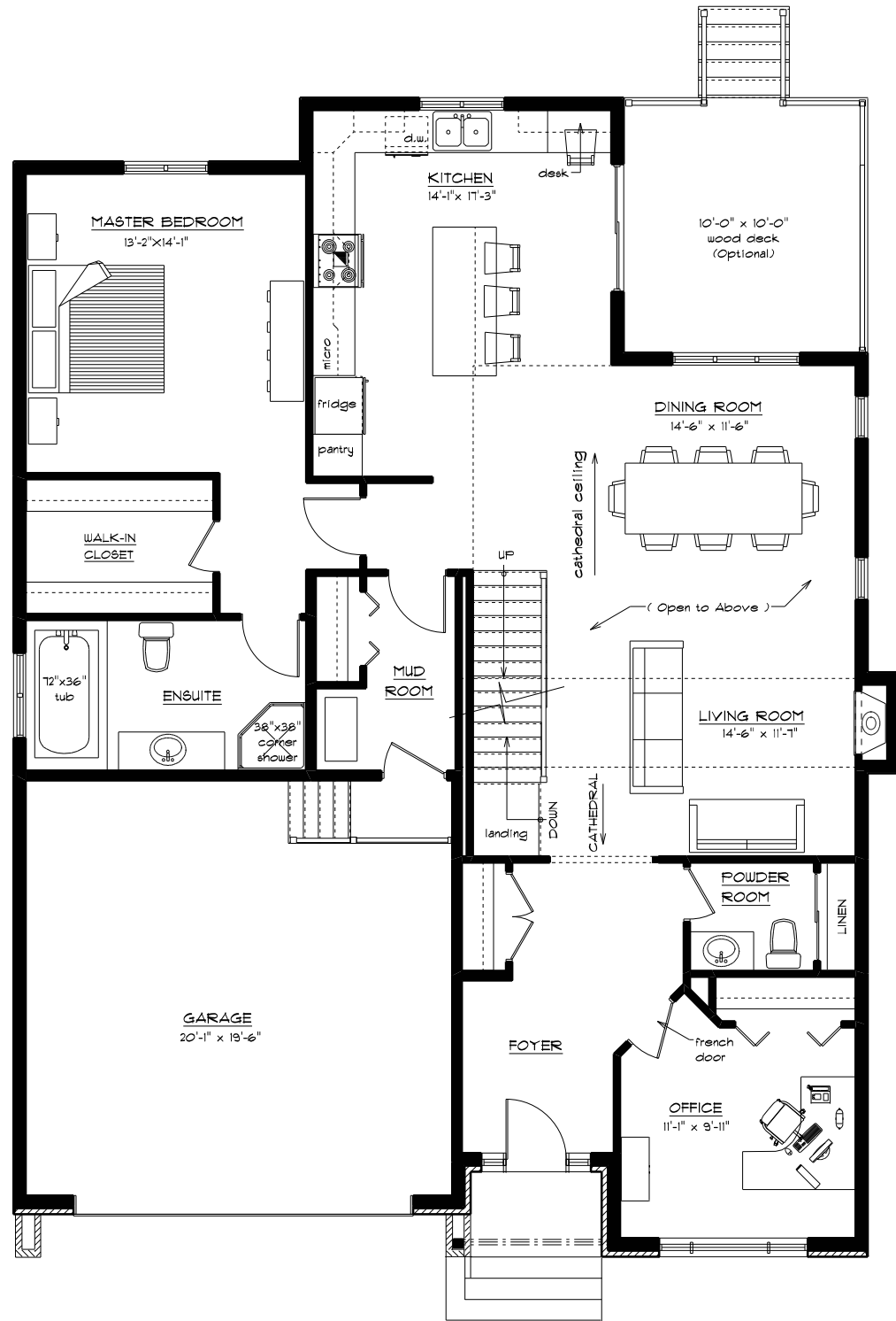
MAIN FLOOR PLAN 1507 sq.ft.
