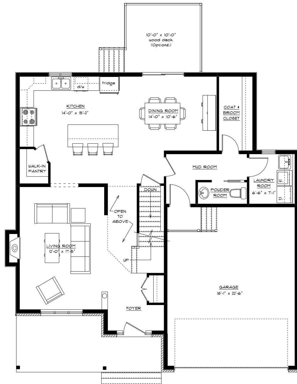
MAIN FLOOR PLAN 1042 sq.ft.
